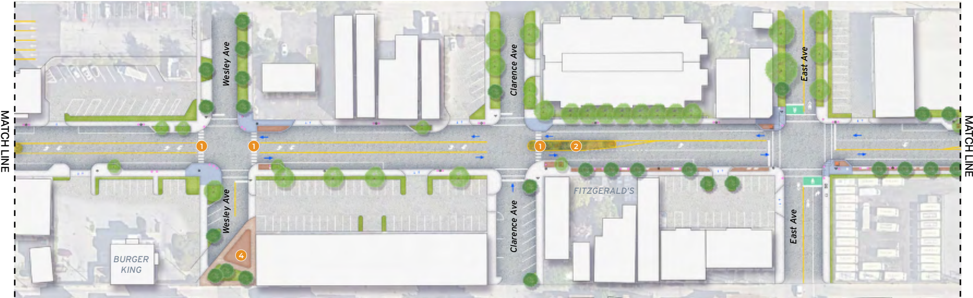
Figure 10: Streetscape Improvements Diagram*
