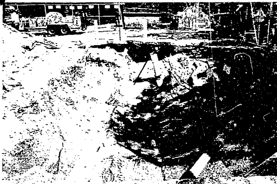
Excavation Zone Following Tank Removal
