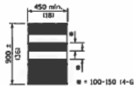
DRUMS AND SAND MODULE IMPACT ATTENUATORS
