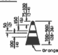
REFLECTORIZED CONES
