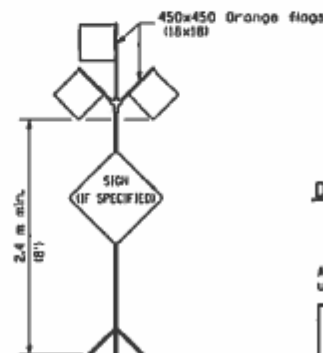
HIGH LEVEL WARNING DEVICE
