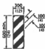
VERTICAL PANELS
