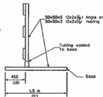
TYPICAL STEEL SUPPORT
