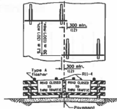
ROAD CLOSED TO ALL THRU TRAFFIC
