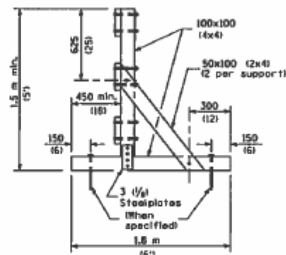
TYPICAL WOOD SUPPORT
